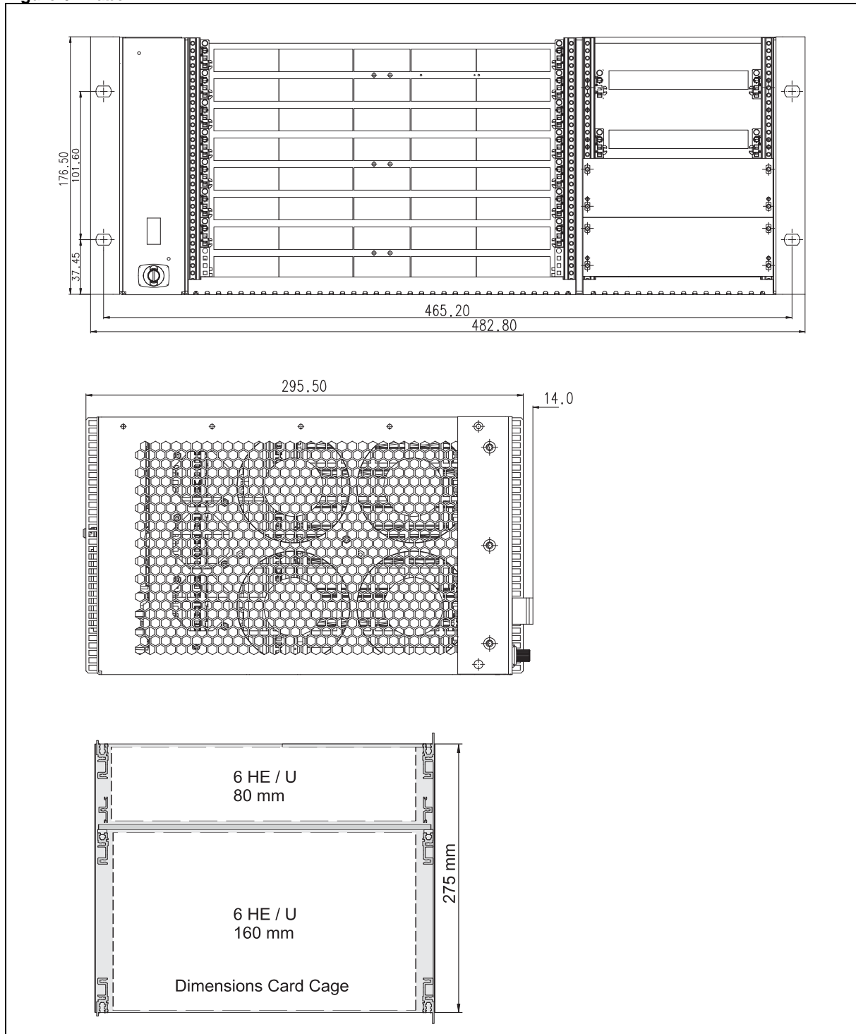
Figure 6: Maße
