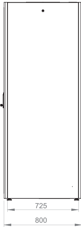
Side view
