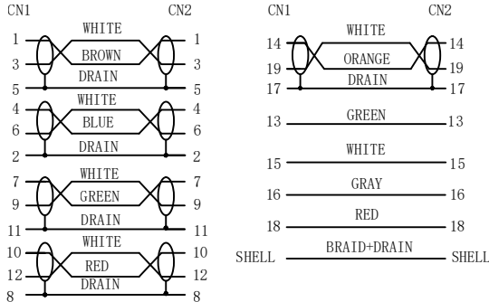
PIN OUT
